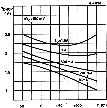
Figure 5: Dropout Voltage vs Junction Temperature
