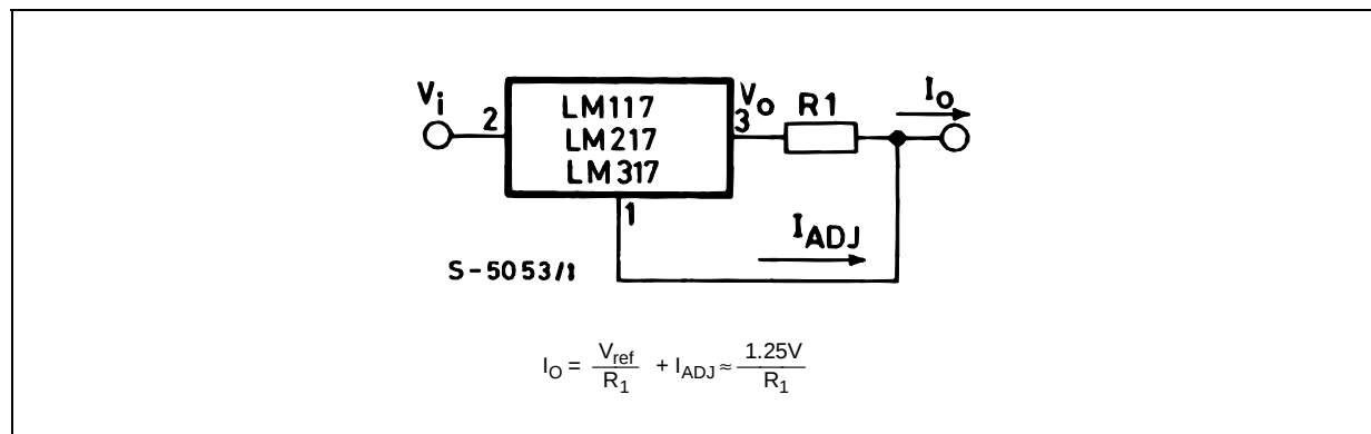
Figure 10: Current Regulator
